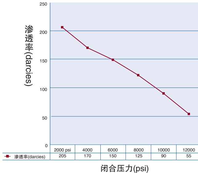
30/50 Interprop 渗透率 (2 lbs/ft 2 @ 250°F)
